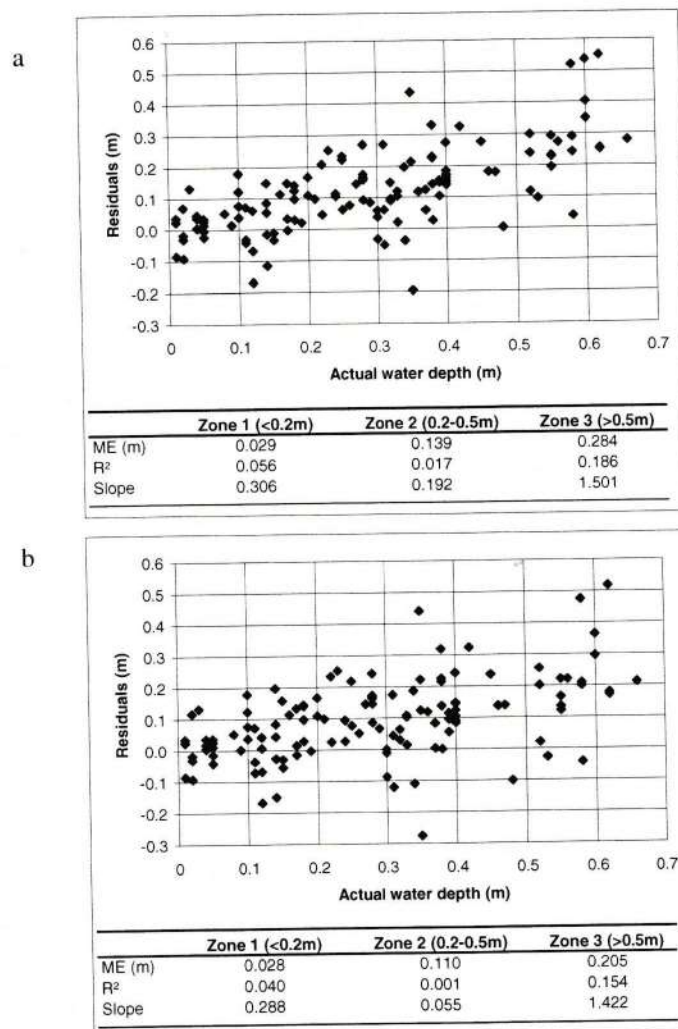
Figure 2: The overall relationship between water depth and error between photogrammetrically-derived and surveyed elevations for (a) uncorrected and (b) corrected DEMs of the three sub-areas.
